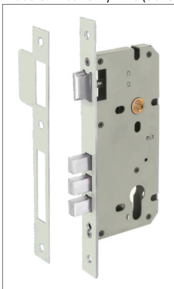
Mortise Lock Body - 3 Sq. Bullet ML 005 SN Economy Zinc (50x85)
