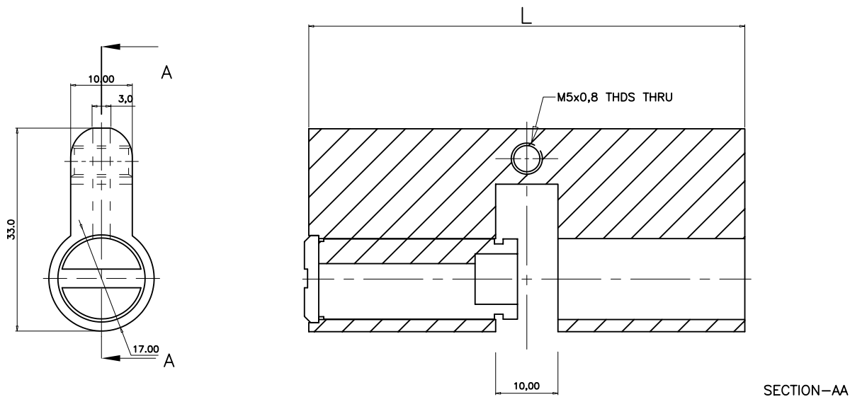
SS Finish Coin & Knob Cylinder Model : RE70C03
