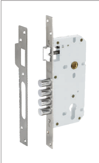
Mortise Lock Body - 4 Bullets ML 001 SS (50mm x 85mm)
